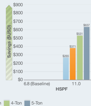
Annual Energy Cost Savings for Heating 6.8-HSPF Baseline*
